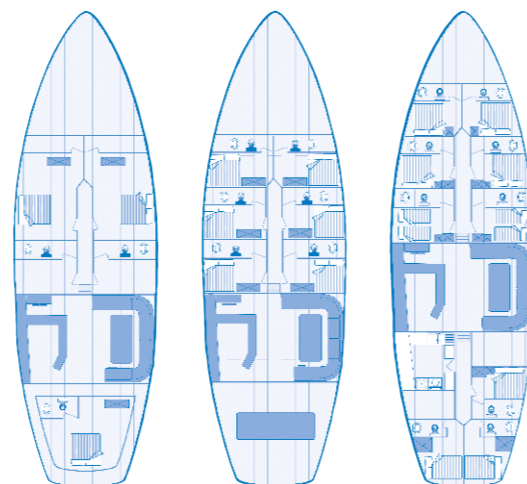
Gulet layout below deck Three Double Cabins Gulet layout below deck Six Double Cabins Gulet layout below deck Eight Double Cabins
